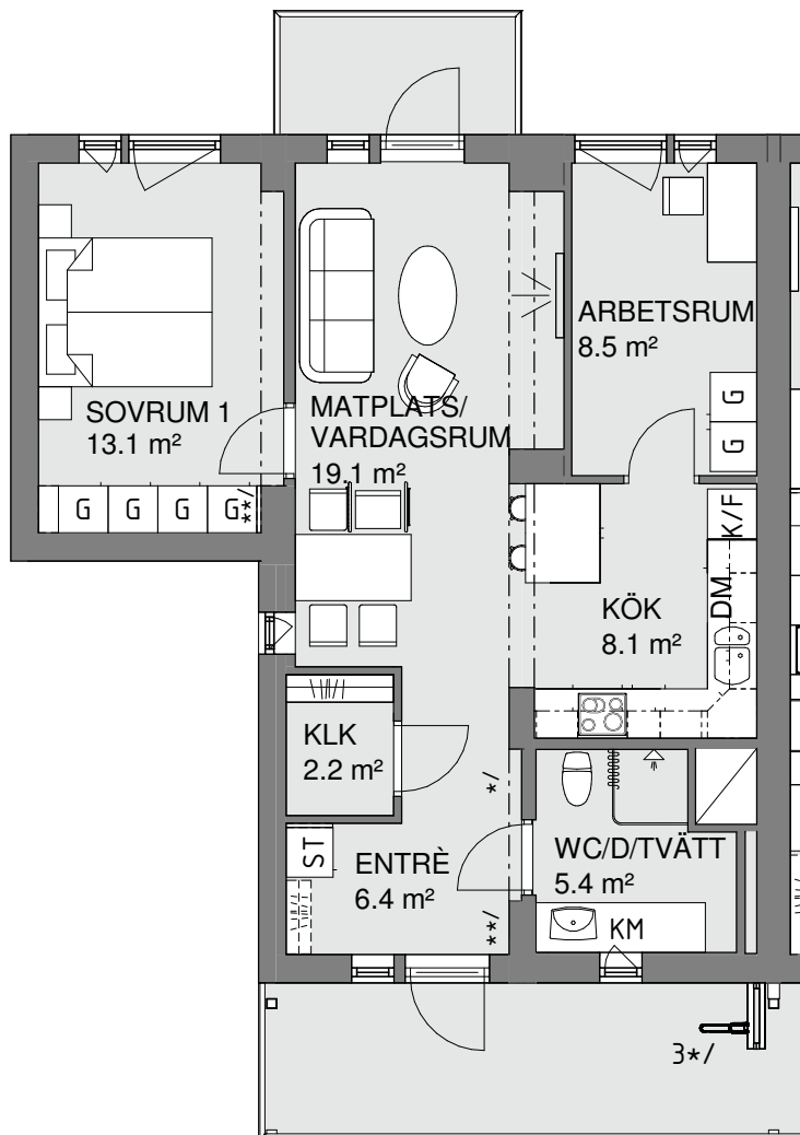
PLAN 2-4
